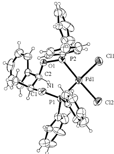
Figure 2. ORTEP view of compound 6b showing the thermal ellipsoids at 30% level of probability
