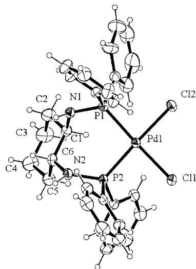
Figure 3. ORTEP view of compound 9b showing the thermal ellipsoids at 30% level of probability
