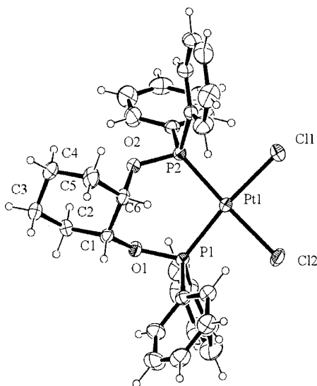
Figure 1. ORTEP view of compound 2a showing the thermal ellipsoids at 30% level of probability
